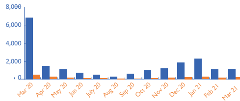
Total Migrants per Month, by Nationality
